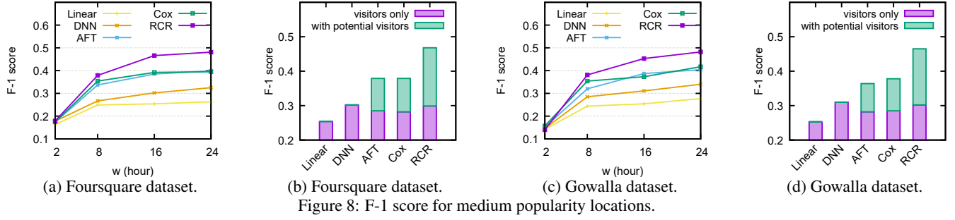
Figure 8: F-1 score for medium popularity locations.
