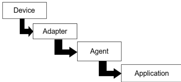
Figure 2. MTConnect Signal Flow from Device to Application
