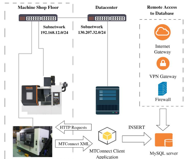
Figure 4. Network Architecture
