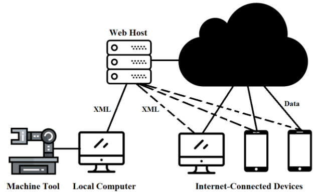
Figure 12. Publishing MTConnect XML on a Host
