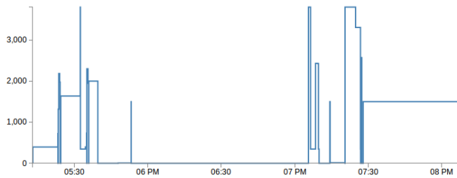
Figure 10. Spindle Speed Chart
