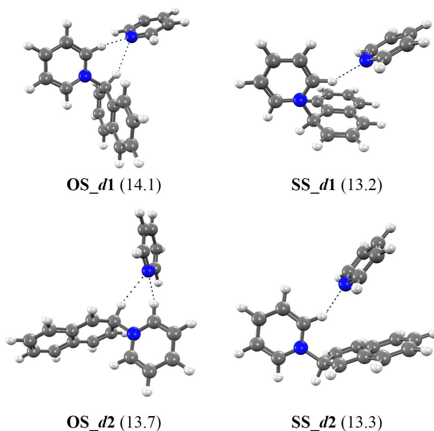
Figure 7. Lowest-energy isomers for the \text{Naph}^{+\bullet}(\text{Pyr})_2 complex with (calculated binding energies in kcal/mol).
