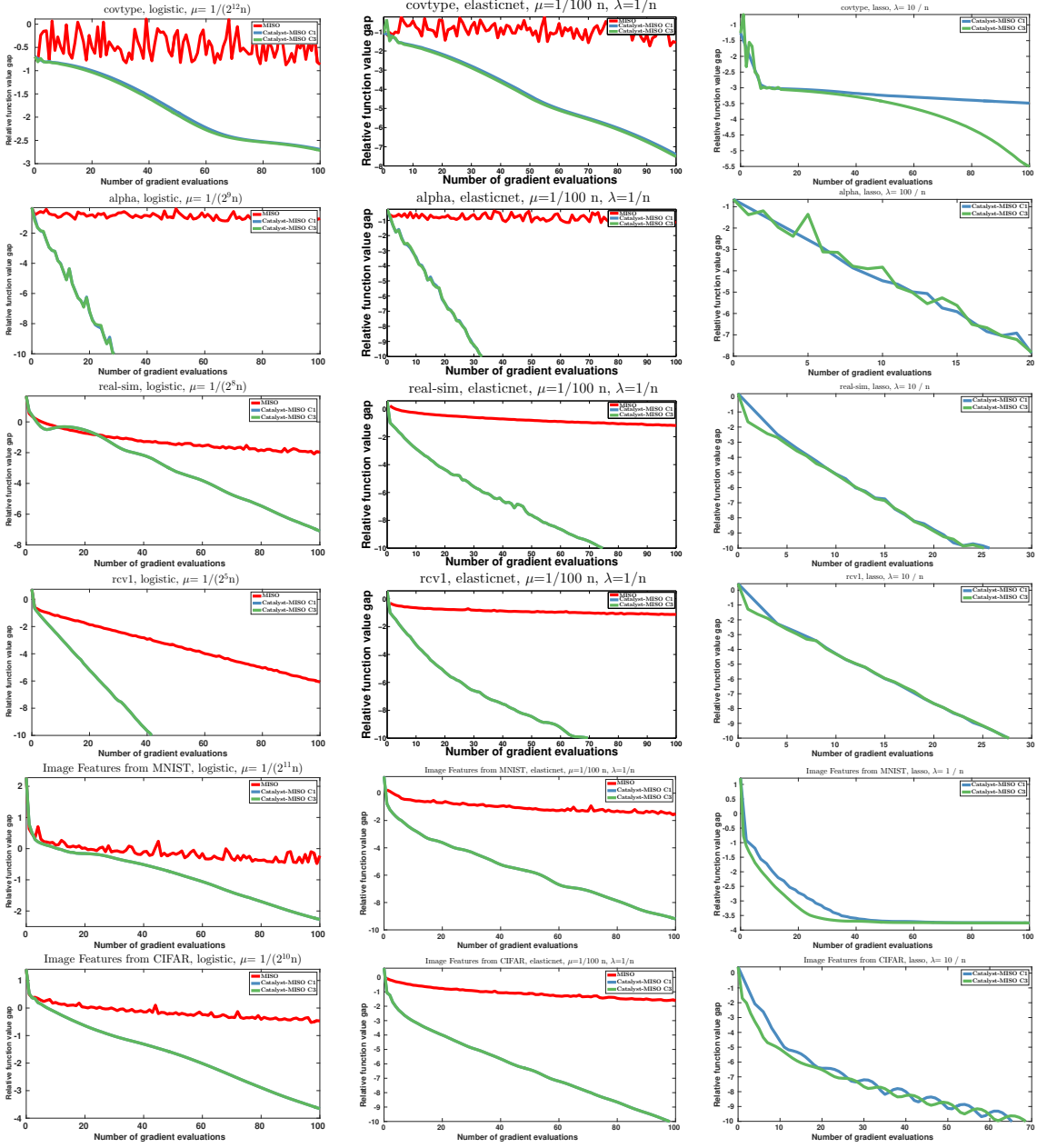
Figure 3: Experimental study of different stopping criterions for Catalyst-MISO, with a similar setting as in Figure 1
