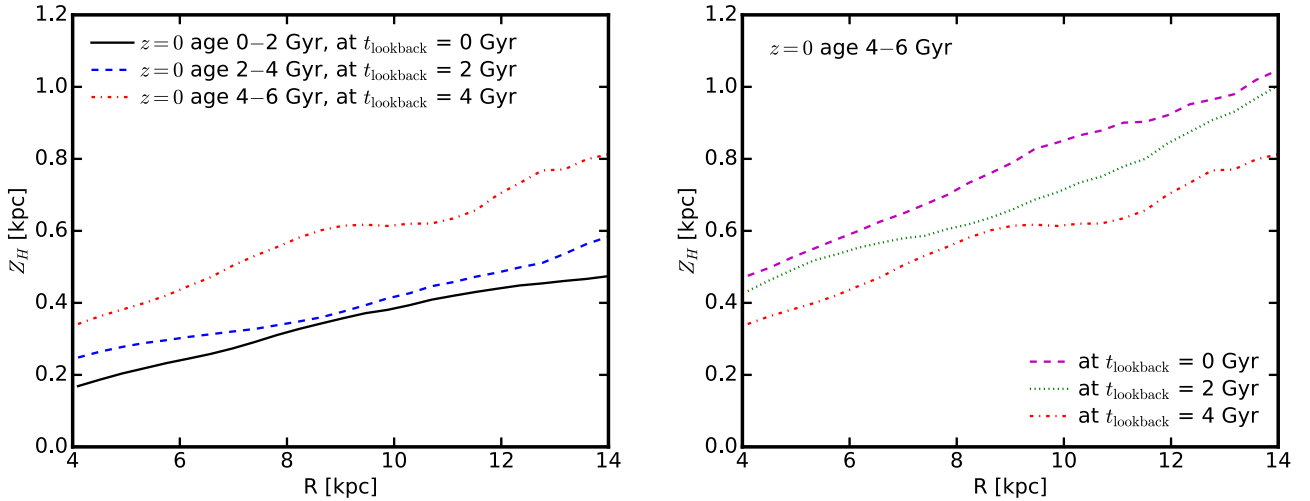
Figure 7. Left-hand panel: scaleheights of stars in three z = 0 age intervals (0–2, 2–4 and 4–6 Gyr), measured at the epoch when the stars formed (labelled by a lookback time). Right-hand panel: the evolution of scaleheights for stars of age 4–6 Gyr at z = 0 , as they would be observed at three different epochs (labelled by a lookback time) after their formation. Stars formed at an early epoch were born in a thicker disc than those formed at later times, because the star-forming disc was more gas-rich and therefore turbulent. The scaleheights of those populations then increase with time due to kinematic heating.
