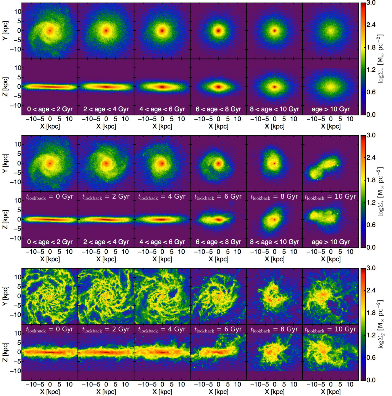
Figure 1. Top panel: morphology of stars in different age intervals at z = 0 . The thickness increases with stellar age, but the scalelength first decreases with stellar age in 0 < \text{age} < 6 Gyr and then increases in \text{age} > 8 Gyr, leaving stars of age \sim 6 Gyr the most radially concentrated (owing to a merger-driven nuclear starburst about this time). Middle panel: morphology of the same stars from each z = 0 age interval in the top panel, but viewed at the epoch when they just formed (labelled by a lookback time) in the galaxy progenitor. Stars younger than 6 Gyr at z = 0 were formed in a relatively calm disc. Stars older than 8 Gyr at z = 0 were formed in a violent, bursty mode, and relax by z = 0 . Bottom panel: morphology of gas, viewed at the same epochs as in the middle panel. At early time, the gas is highly irregular and chaotic. By t_{\text{lookback}} \sim 6 Gyr ( z \sim 0.7 ), the gas eventually formed a disc.
