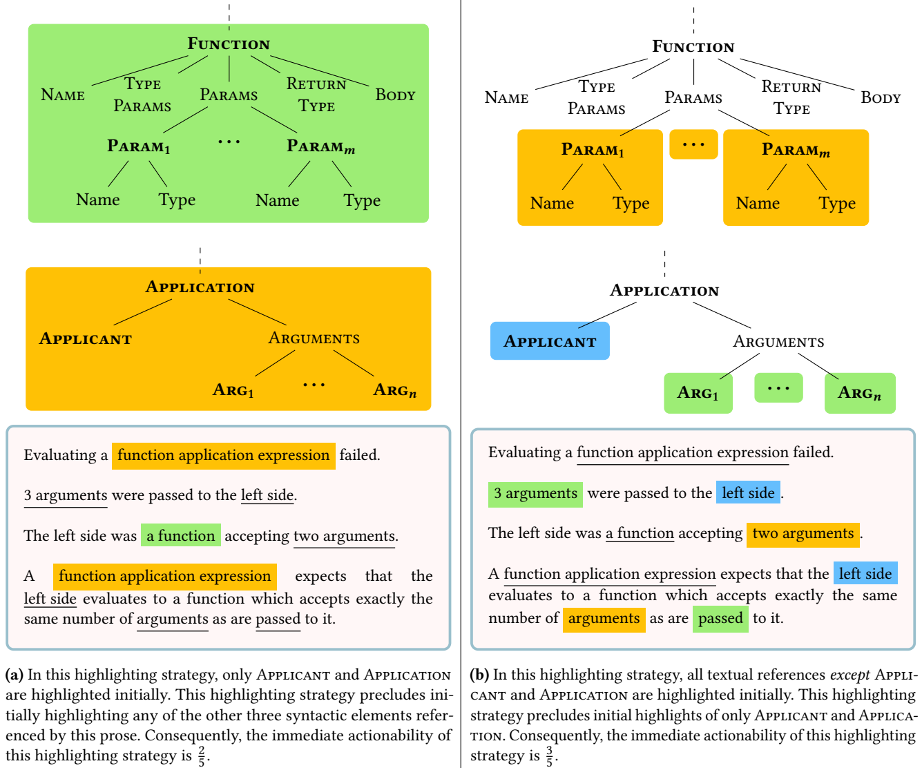
Figure 4. Two potential highlighting strategies for an arity-mismatch error. From top to bottom: the highlighting plan depicted on the P-AST of the definition site, the highlighting plan depicted on the P-AST of the application site, the consequences of the program highlighting plan on the highlighting of the error report prose. The caption of each highlighting plan describes the plan and quantifies its impact on the highlighting of the prose with an immediate actionability score. The colors in this diagram reflect the initially highlighted set of phrases and program fragments. The underlined phrases indicate the references to syntactic elements that are highlighted on-demand.
