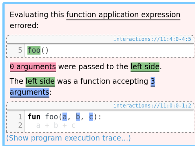
Figure 5. An error report for ARITY-MISMATCH with the textual reference to the actual parameters highlighted in pink. The program source does not contain a corresponding highlight because the source contains no parameters on which a highlight can be displayed.
