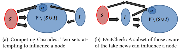
Figure 1: Fundamental distinction between FActCheck and Competing Cascades. FActCheck enforces the constraint that the news must pass through the set I .
