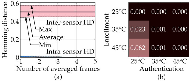
Figure 7: Uniqueness and robustness evaluation: (a) Intra- and inter-sensor HDs for varying number of averaged frames ( N_f ). (b) Intra-sensor HDs for varying enrollment and authentication temperatures.
