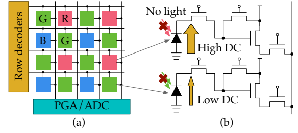
Figure 1: (a) Architecture of a CMOS image sensor with the Bayer pattern color filter. (b) Dark current (DC) variation between pixel sensors when there is no incoming light.
