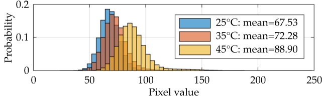
Figure 2: Distributions of pixel values of the averaged dark frames of a Sony IMX377 at different temperatures.
