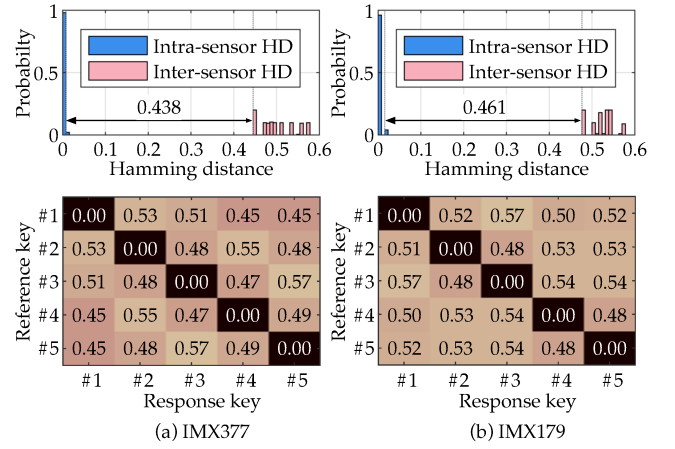
Figure 8: Intra- and inter-sensor HD distributions and average HD matrices of (a) IMX377 and (b) IMX179.
