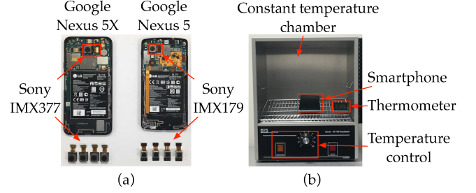
Figure 5: Experimental setup: (a) Smartphones and image sensors. (b) Constant temperature chamber used for temperature control.
