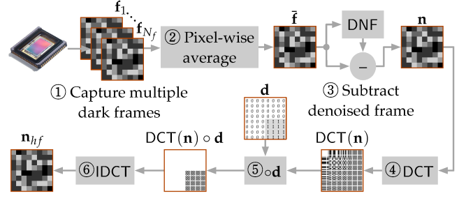
Figure 3: DSNU fingerprint extraction procedure.
