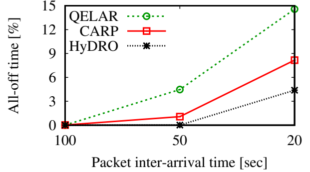
Figure 3: All-off time.
