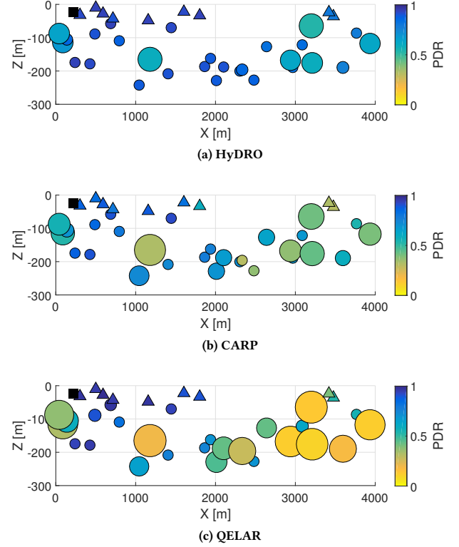
Figure 6: A vertical view of a network topology with 40 nodes and high traffic: Joint PDR and all-off time.
