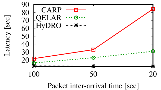
Figure 4: End-to-end latency.
