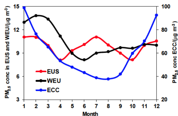
Figure 5. Monthly mean surface \text{PM}_{2.5} concentrations during 2007–2016 in three target regions. The numbers of observational sites included in averaging are 225, 52, and 496, in the EUS, WEU, and ECC regions. Note the different scales on the y axes for EUS/WEU and ECC.
