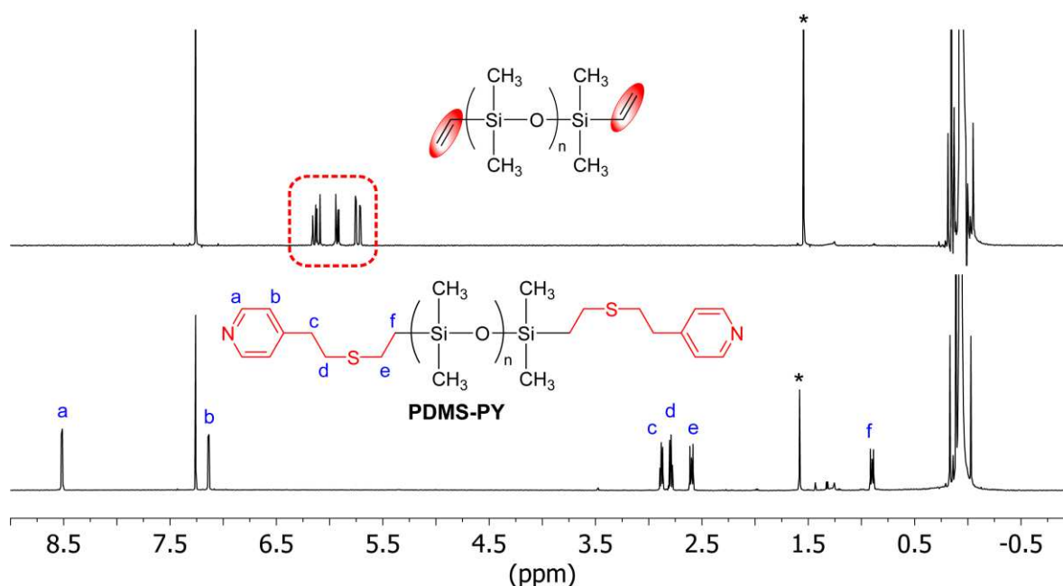
Figure 2. ^1\text{H} NMR spectra comparison (25 °C, \text{CDCl}_3 ) of vinyl-terminated telechelic PDMS commercial sample (top), and after installation of pyridyl end-group ( PDMS-PY , bottom) via “click” reaction. (* = \text{H}_2\text{O} trace from “wet” \text{CDCl}_3 ).
