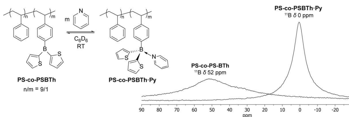
Figure 3. Stoichiometric reaction between PS-co-PS-BTh and pyridine and resulting ^{11}\text{B} NMR spectra.
