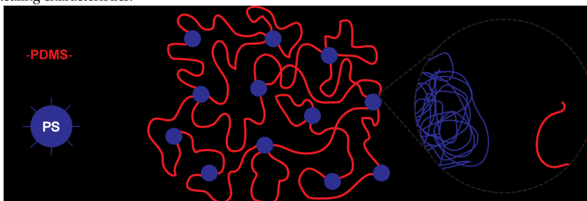
Figure 1. Schematic representation of the proposed crosslinked supramolecular network in the PS/PDMS blend promoted by Lewis-acid/Lewis-base pairs (LA = Lewis acid, LB = Lewis base).
