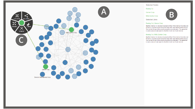
Figure 2: Tangraphe User Interface. (a) Visualization canvas, (b) Details panel and (c) Radial context menu
