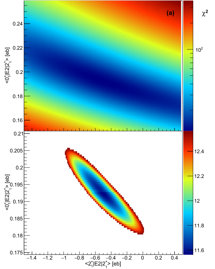
Fig. 3. \chi^2 surfaces in ^{22}\text{Mg} determined through a comparison of calculated Coulomb-excitation yields and experimental yields using GOSIA2 [41]. (a) Total \chi^2 surface for the \langle 0_1^+ || E2 | 2_1^+ \rangle and \langle 2_1^+ || E2 | 2_1^+ \rangle matrix elements. (b) As (a) but within the \chi_{\min}^2 + 1 ( 1\sigma ) limit, demonstrating the preference for a negative \langle 2_1^+ || E2 | 2_1^+ \rangle matrix element.
