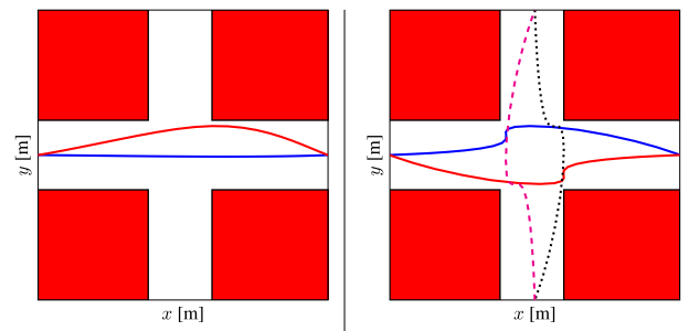
Fig. 11. Workspace and trajectories under reach avoid specifications for a two-robot scenario (left) and a four-robot scenario (right).
