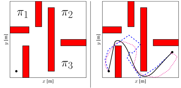
Fig. 10. (Left) Workspace used in our experiments; (right) trajectories generated by the SMC-based (black), Synergistic RRT (dashed blue), and Synergistic EST (dotted red) motion planners for the double integrator dynamics.
