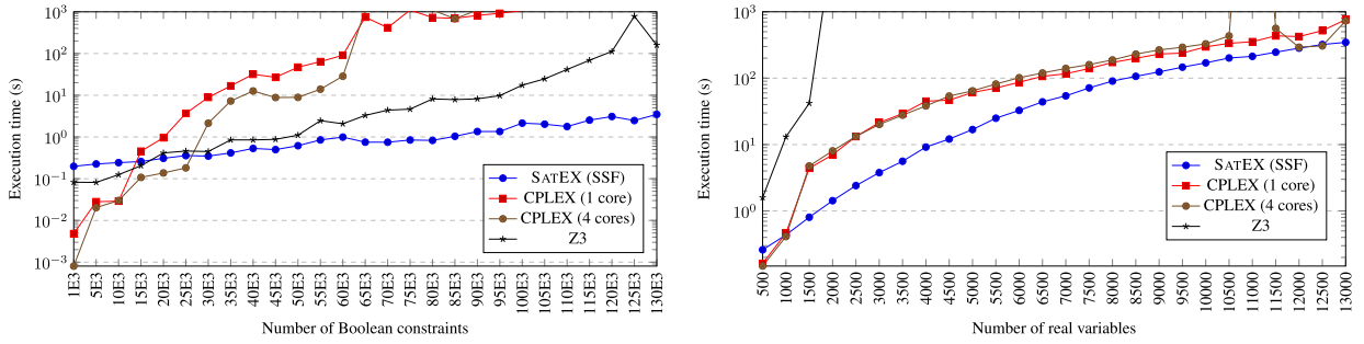
Fig. 6. Execution time on SMC problem instances, when the number of Boolean constraints increases for a fixed number of 100 real variables (left side) and when the number of real variables increases for a fixed number of 7000 Boolean constraints (right side).
