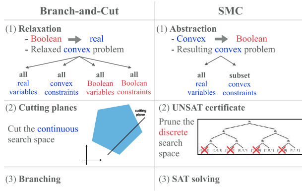
Fig. 2. Comparison between mixed integer convex programming (MICP) based techniques and the SMC approach.
