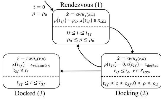
Fig. 4. Hybrid system representation of the ARPOD mission.
