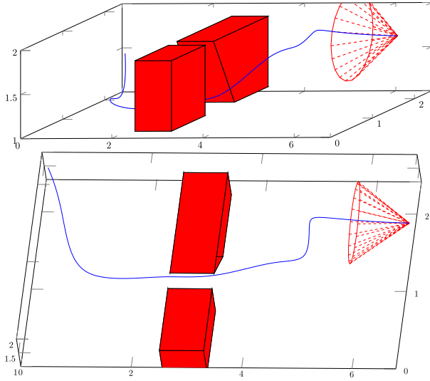
Fig. 13. Trajectory generated by SatEX for the ARPOD test-case (all units are in kilometers). The different views show the shape of the obstacles and the LOS cone (top) as well as the position of the start and docking points (bottom).
