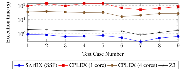
Fig. 7. Execution time on UNSAT SMC instances due to UNSAT Boolean constraints: the number of Boolean clauses varies from 225 to 960, while the number of real variables is fixed at 500.
