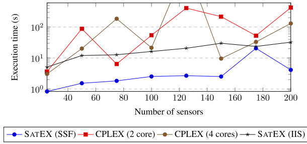
Fig. 8. Execution time on instances of the secure state estimation problem when the number of sensors increases. Z3 exceeds a 600-s timeout in all benchmarks.
