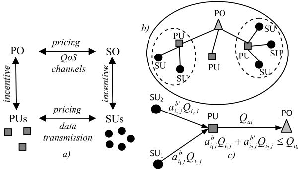
Fig. 1. Cognitive Dynamic Network Architecture. (a) Data and Spectrum Trading. (b) PU-SU association. (c) Data Forwarding.
