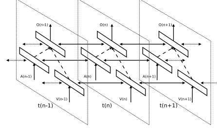
(a) BRNN framework [4]
