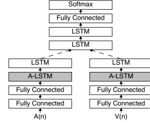
(b) Proposed BRNN with A-LSTM
