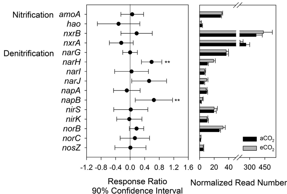
Fig. 3. Response ratio analysis (90% confidence interval) and the normalized abundance of gene families involved in nitrification and denitrification processes. The total number of reads in each sample was normalized to one million. ** represents significant changes at 95% confidence interval.
