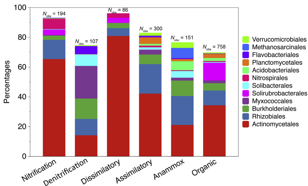
Fig. 6. Taxonomic groups involved in major nitrogen cycling processes. Only the top five most abundant microbial orders and the ones with >3% relative abundance are shown in the color legends. The numbers above each bar represent the observed number of microbial species in their corresponding processes. (For interpretation of the references to colour in this figure legend, the reader is referred to the web version of this article.)
