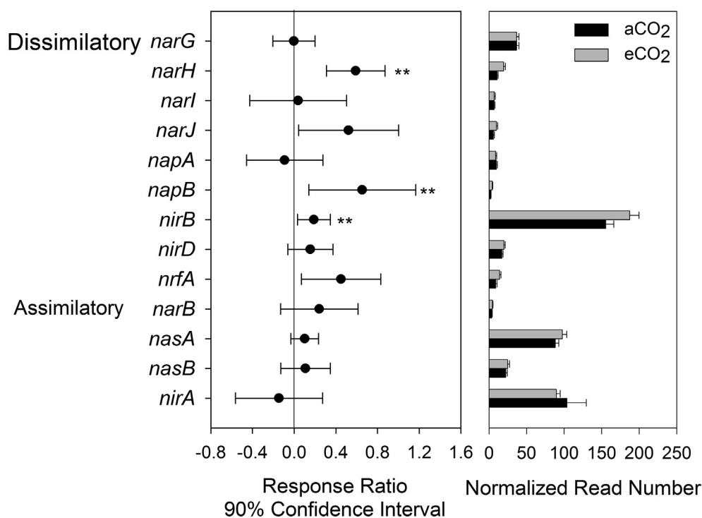
Fig. 4. Response ratio analysis (90% confidence interval) and the normalized abundance of gene families involved in dissimilatory and assimilatory nitrate reduction processes. Significantly increased abundances of gene families for dissimilatory nitrate reduction were detected, but not for assimilatory nitrate reduction. The total number of reads in each sample was normalized to one million. ** represents significant changes at 95% confidence interval.
