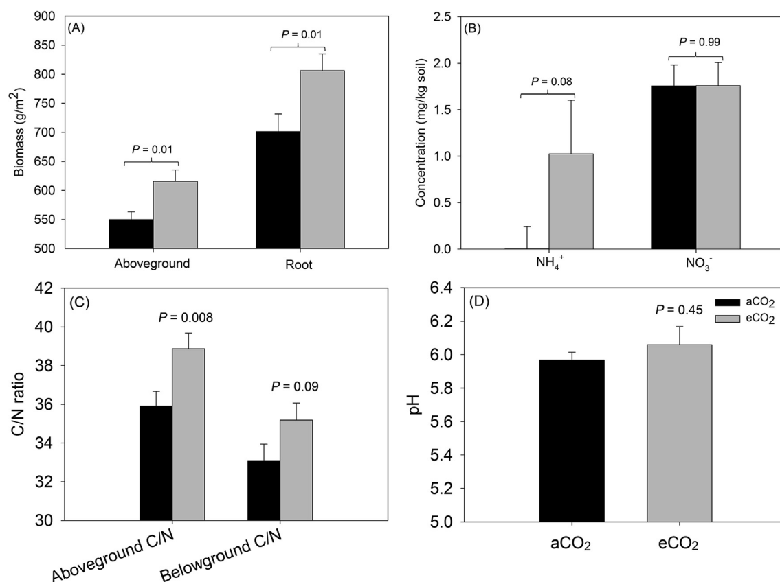
Fig. 1. Elevated CO 2 effects on plant biomass (A) and soil nitrogen (NH 4 + and NO 3 - ) (B). Both aboveground and root biomass were significantly stimulated under eCO 2 treatment. Long-term eCO 2 also significantly stimulated ammonification in the soil, but not nitrification. Data from year 2005–2009 were collected and analyzed by the Student's t -test.
