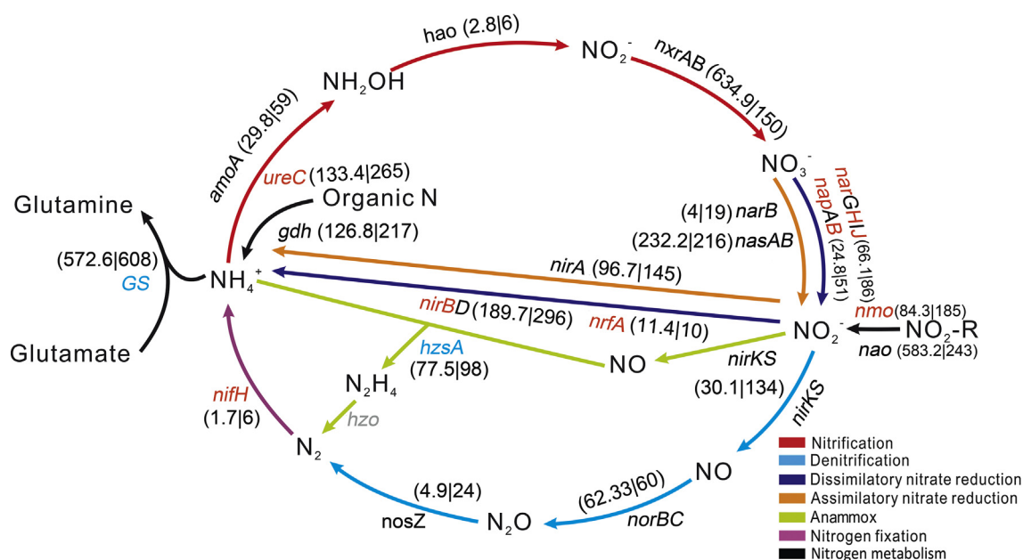
Fig. 2. An overall schema illustrating the nitrogen cycling processes in the grassland ecosystem as well as their responses to long-term eCO 2 . Under eCO 2 , the gene families marked in red indicate a significantly increased abundance, the gene families in light blue indicate a significantly decreased abundance, and the gene families in black indicate no significant changes. The numbers in the brackets beside each gene represent the normalized abundance (left) and observed number of microbial species (right) for the gene family. Different colors represented different functional processes. (For interpretation of the references to colour in this figure legend, the reader is referred to the web version of this article.)
