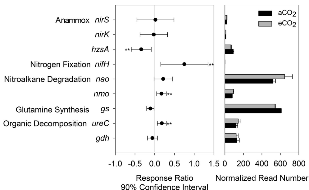
Fig. 5. Response ratio analysis (90% confidence interval) and the normalized abundance of gene families involved in anammox, N 2 fixation, organic N metabolism, and glutamine synthesis processes. Significantly changed abundances of gene families for anammox, N 2 fixation, and organic N metabolism were detected. The total number of reads in each sample was normalized to one million. ** represents significant changes at 95% confidence interval.
