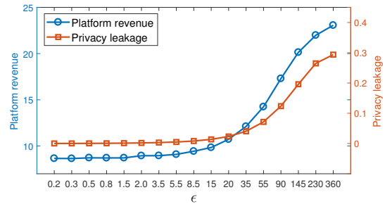
Fig. 3. Impact of privacy budget \epsilon to platform revenue and privacy leakage.
