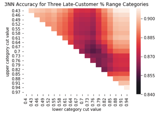
Figure 18: Accuracy Heat Map for Three Customer Experience Classes
