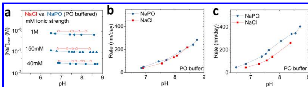
Figure 5. Dependence of TG-SiO 2 dissolution on anion type. (a) Na + concentrations in solutions of NaCl and Na 2 HPO 4 /NaH 2 PO 4 (NaPO). (b) Dissolution rates in solutions with 40 mM ionic strength. (c) Dissolution rates in solutions with 150 mM ionic strength.
