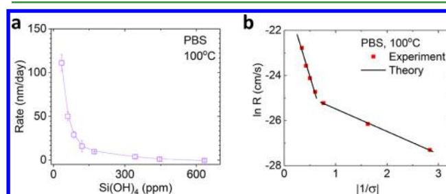
Figure 3. Effects of silicic acid on dissolution of TG-SiO 2 . (a) Effect of silicic acid concentration on dissolution rate in PBS. (b) Comparisons to a polynuclear dissolution model.
