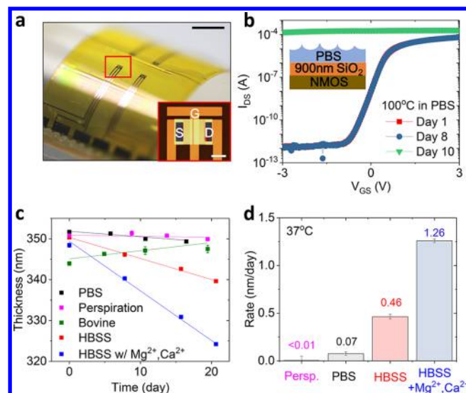
Figure 1. Flexible electronics encapsulated with thermally grown silicon dioxide (TG-SiO 2 ) and dissolution of TG-SiO 2 due to immersion in simulated biofluids at 37 °C. (a, b) Demonstration of electronic devices and flexible electronic systems encapsulated with TG-SiO 2 . (a) Optical images of flexible n-type metal-oxide-semiconductor (NMOS) transistors (scale bar: 1 cm (black), 200 μm (white, inset)). (b) Results of soak tests of NMOS in PBS solutions at 100 °C. (c) Change in thickness of TG-SiO 2 as a function of time of immersion in simulated biofluids. (d) Measured dissolution rates (nm/day) for these fluids.
