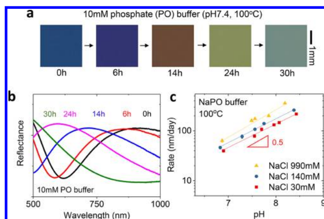
Figure 2. Effects of ion concentration and pH on dissolution of TG-SiO 2 . (a) Optical images of TG-SiO 2 collected at several times of immersion in 10 mM sodium phosphate (Na 2 HPO 4 /NaH 2 PO 4 NaPO) solution (pH 7.4) at 100 °C. (b) Reflectance curves at different times. (c) Effects of pH and NaCl concentration on the dissolution rate.
