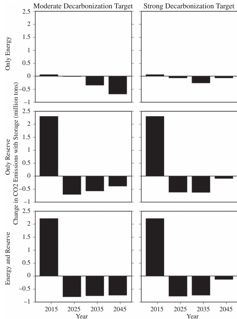
Figure 5. Change in system CO 2 emissions with storage versus without storage under the moderate (left) and strong (right) decarbonization targets when storage participates in only energy (top row), only reserve (middle row), or energy and reserve (bottom row) markets. Positive values indicate storage increases CO 2 emissions.
