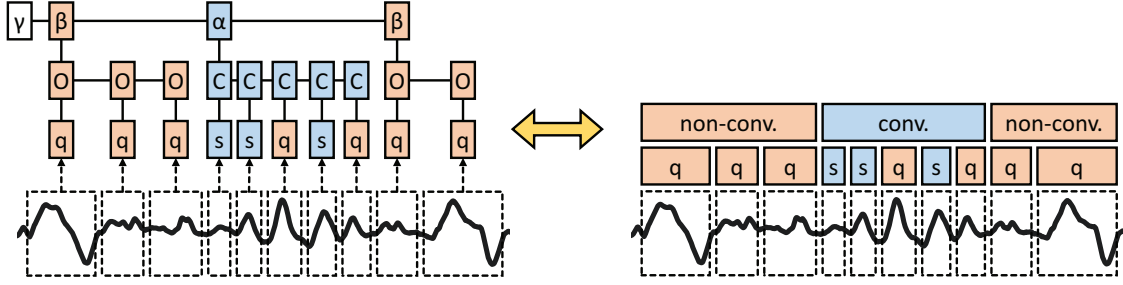
Fig. 6. An example parse (left) using the grammar described in equation 4. Also shown is the mapping from the parse to a labeled segmentation (right) where q and s stand for quiet and speaking respectively.
