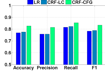
Fig. 10. Cycle labeling performance of different models on training data. LR: Logistic Regression, LC-CRF: Linear Chain CRF, CRF-CFG: CRF with Context Free Grammar.
