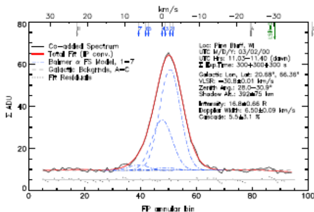
Figure 2. PBO FPI coadded ( \times 3 ) geocoronal Balmer \alpha spectrum (black), and the seven fine structure components (blue, dashed) comprising the total cascade model fit (red). Two atmospheric (A and B) and one Galactic background (C) component were also accounted for in the fits; residuals are plotted beneath. Components from Table 2 are listed along the top abscissa, where the kilometers per second scale is relative to component 4. These coadded spectra were obtained on 2 March 2000 at Pine Bluff Observatory, WI, near solar maximum over several tens of minutes toward a constant-viewed low-emission Galactic region, just before sunrise. The shadow altitude (and zenith angle) at the beginning of the first coadded observation was 467 km ( 28^\circ ), and by end of the last observation, it was 317 km ( 30.9^\circ ).
