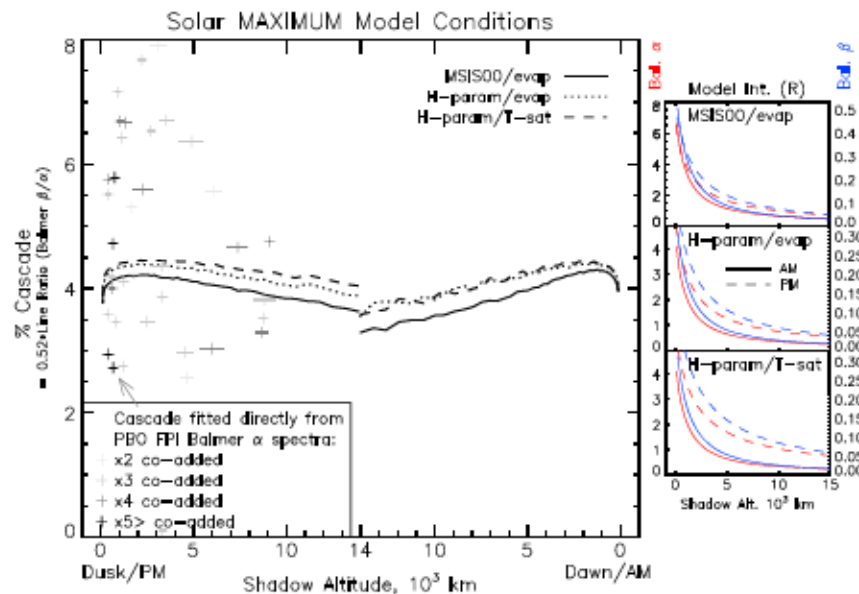
Figure 7. AM and PM solar maximum modeled line ratio (expressed as cascade) versus shadow altitude, using three different thermosphere and exosphere model parameterizations (refer to text and Table 5). All three modeled line ratios have nearly equivalent, steeply rising low shadow altitude peak location and magnitudes, followed by broad negative curvature toward deeper shadow altitudes. A similar behavior is mildly apparent in the overplotted darker crosses for cascade contributions as determined from coadded fits to high-resolution Balmer \alpha line profiles. In the right inset plots, for each modeled Balmer \beta/\alpha line ratio, the model intensities ( R ) are plotted where blue (red) traces are for Balmer \beta (Balmer \alpha ) with respect to the right (left) scaled axis.
