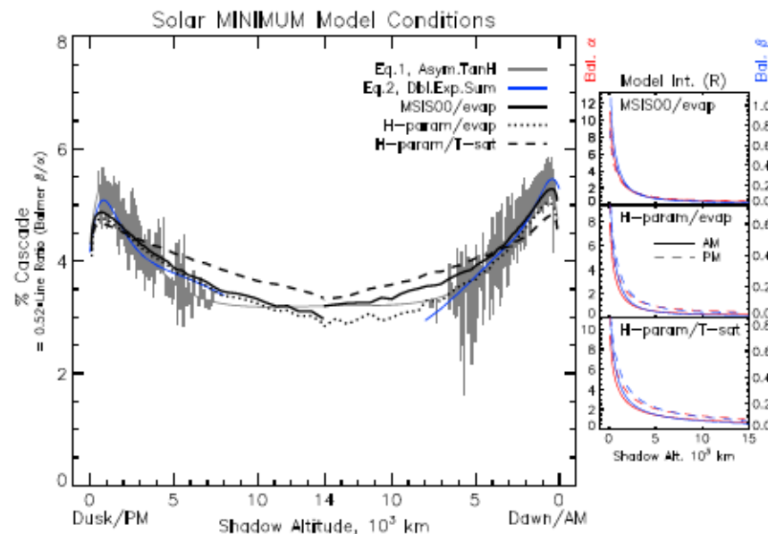
Figure 8. AM and PM solar minimum modeled line ratio (expressed as cascade) versus shadow altitude, using different thermosphere and exosphere model parameterizations (refer to text and Table 5). All three modeled line ratios have nearly equivalent, steeply rising low shadow altitude peak location and magnitudes, followed by broad positive curvature toward deeper shadow altitudes. A similar behavior is seen in the overplotted gray and blue cascade curves determined from WHAM observations (refer to Figure 5). For right inset plots, refer to Figure 7 caption.
