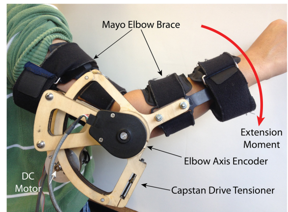
Fig. 2 Motorized elbow brace. Right-handed elbow brace with motorized capstan drive. The brace produced an extension moment about the elbow proportional to force measured by the gripper
