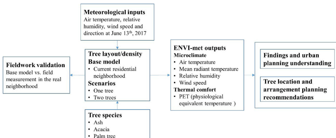
Fig. 2. Methodology framework.
