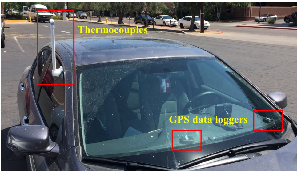
Fig. 3. Vehicle-based air temperature thermocouples and GPS data logger placement for traverse measurements.
