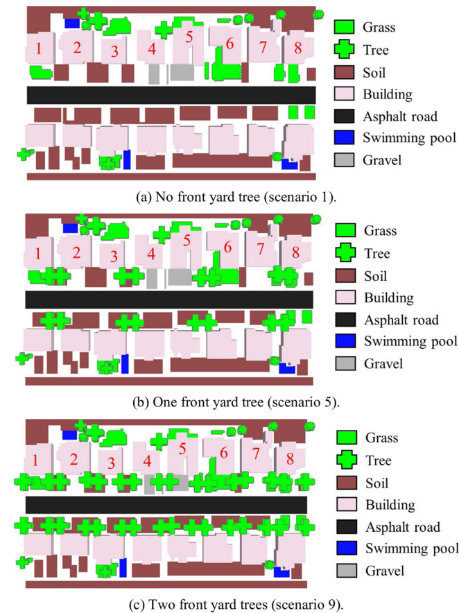
Fig. 6. Simulated tree locations and arrangement scenarios (selected scenarios).
