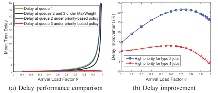
Fig. 5: Delay performance in the asymmetric setup
