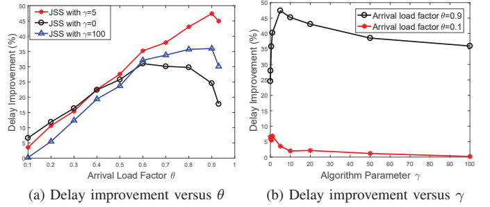
Fig. 6: Job delay improvement ratio of JSS algorithm
