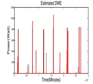
Fig. 11. Dishwasher Reconstruction
