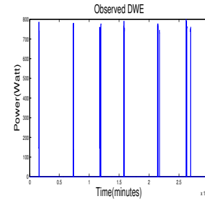
Fig. 10. Dishwasher Observed
