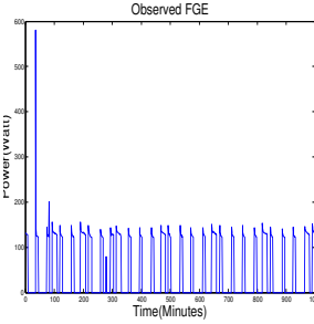
Fig. 8. Refrigerator Observed
