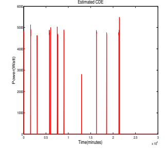
Fig. 7. Dryer Reconstruction
