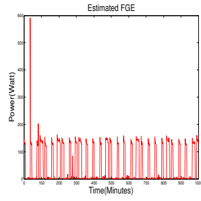
Fig. 9. Refrigerator Reconstruction
