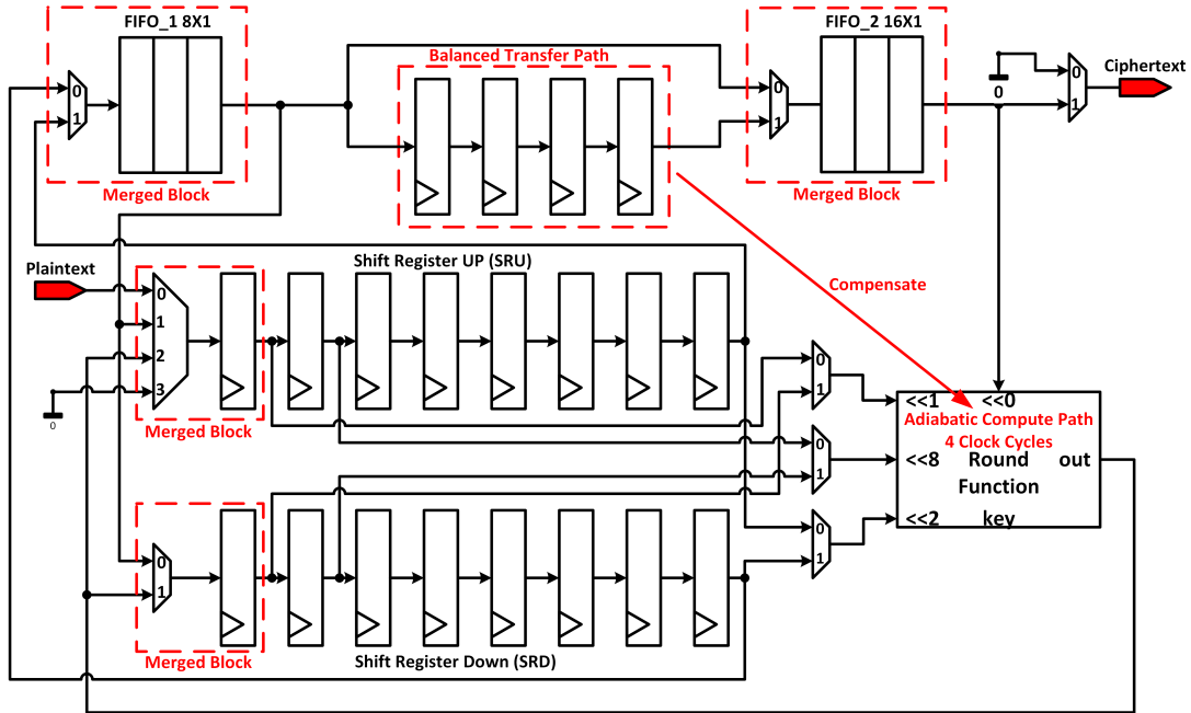
Fig. 8: Proposed adiabatic architecture for round function of the bit-serialized SIMON32/64 cipher.
