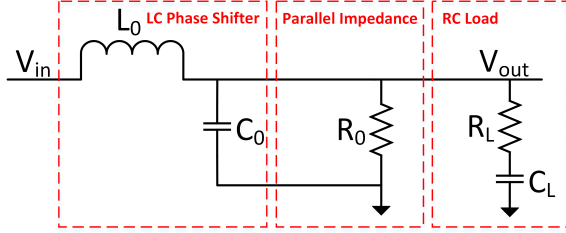
Fig. 5: An RLC model of an LC phase shifter with load.
