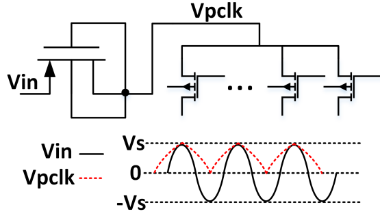
Fig. 7: Schematic of a diode-connected MOS signal shaper.
