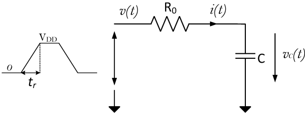
Fig. 2: Equivalent RC circuit to determine the energy loss in charge-recycling adiabatic logic.
