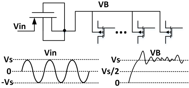
Fig. 4: Schematic of a diode-connected MOS peak detector.
