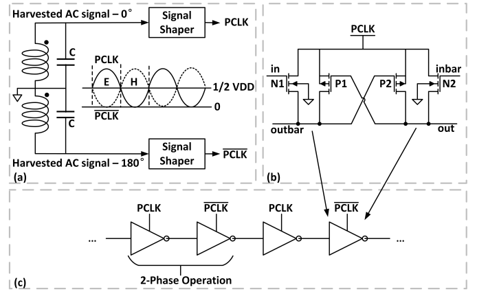
Fig. 6: Proposed PAL based AC computing system: (a) 2-phase power-clock generation and signal waveform, (b) schematic of PAL based inverter, (c) chains of PAL logic gates.
