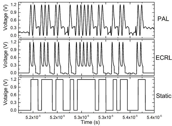
Fig. 11: Simulated output waveforms of the SIMON32/64 cipher blocks in each approach, demonstrating functional verification.
