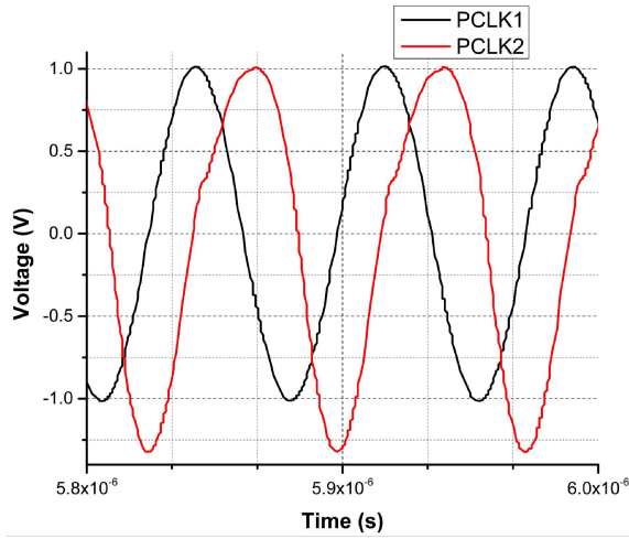
Fig. 10: Simulated output waveforms of the LC phase shifter, illustrating the 90^\circ phase difference.
