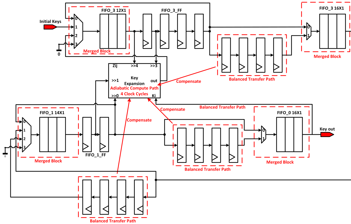
Fig. 9: Proposed adiabatic architecture for key expansion of the bit-serialized SIMON32/64 cipher.
