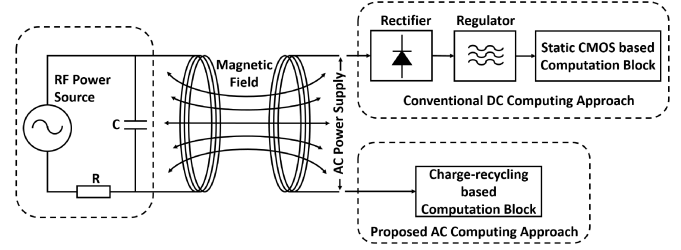
Fig. 1: Proposed AC computing methodology for RF powered IoT devices versus conventional method with rectifier and regulator.
