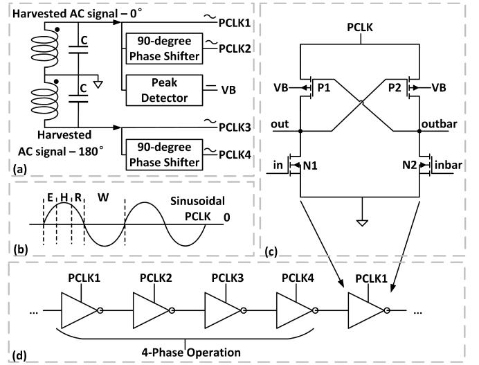
Fig. 3: Proposed ECRL based AC computing system: (a) 4-phase power-clock generation, (b) power-clock signal waveform and 4 operation intervals, (c) schematic of ECRL based inverter, (d) chains of ECRL logic gates.
