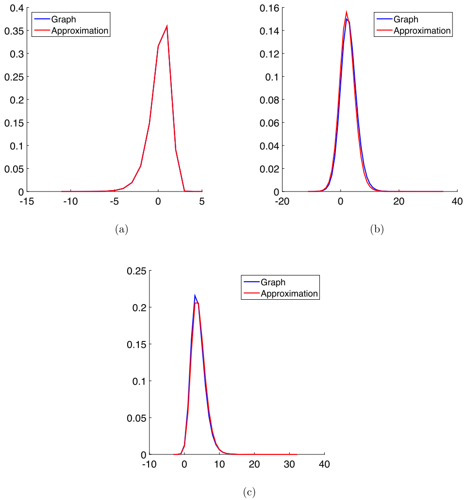
FIG. 1. Hopcount probability mass function compared to the approximation provided by Theorem 2.5 for: (a) a 3-regular bi-degree sequence; (b) a bi-degree sequence generated by the i.i.d. algorithm with independent in- and out-degrees; and (c) a bi-degree sequence generated by the i.i.d. algorithm with dependent in- and out-degrees. The Kolmogorov–Smirnov distance in each case is: (a) 1.3 \times 10^{-4} , (b) 0.0583, and (c) 0.0353. In all cases the graphs had n = 10^6 nodes.
