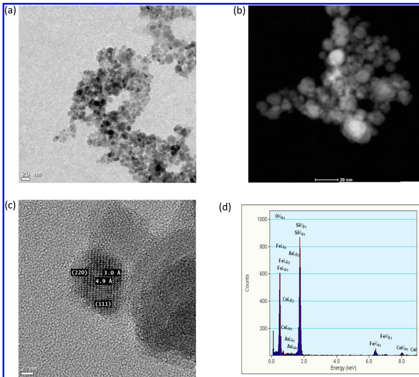
Figure 1. (a) Low resolution TEM image of HA-MNPs, (b) STEM-HAADF image of As(III)-HA-MNPs, (c) HRTEM image of As(III)-HA-MNPs, and (d) EDS spectra of As(III)-HA-MNPs.
