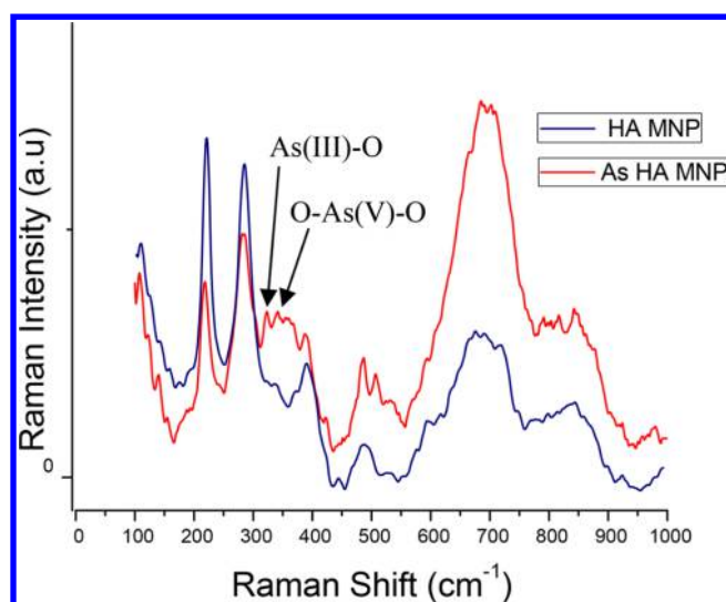
Figure 2. Raman spectra of HA-MNPs and As(III)-HA-MNPs.
