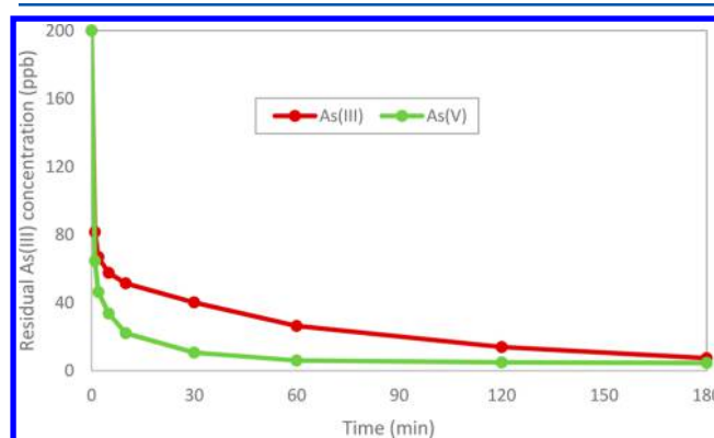
Figure 3. Comparison of adsorption kinetics of As(III) and As(V) on HA-MNPs. [As(III)] 0 = 200 ppb, [As(V)] 0 = 200 ppb, pH = 6.6, HA-MNP dose = 0.2 g/L, temperature = 25 °C.
