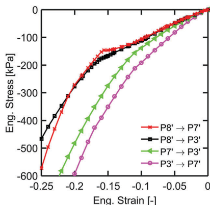
Fig. 8 Stress–strain relation obtained from FE simulation using unit-cells enclosed by lattice vectors \mathbf{a}_1 and \mathbf{a}_2 . The radius ratio is \chi = 0.4 .
