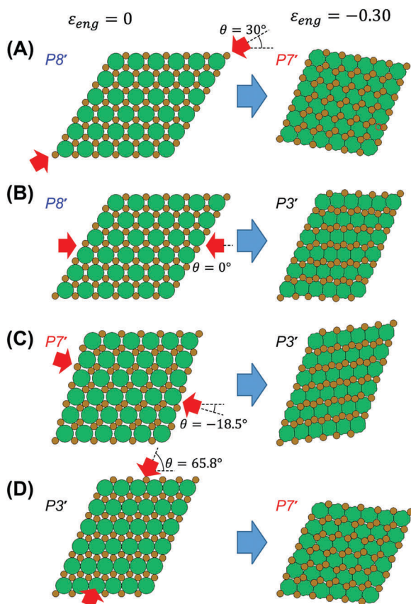
Fig. 9 FE simulation results using unit-cells enclosed by lattice vectors 5\mathbf{a}_1 and 5\mathbf{a}_2 . The radius ratio is \chi = 0.4 . (A) P8' to P7' . (B) P8' to P3' . (C) P7' to P3' . (D) P3' to P7' .
