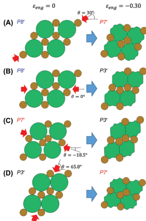
Fig. 7 FE simulation results using unit-cells enclosed by lattice vectors \mathbf{a}_1 and \mathbf{a}_2 . The radius ratio is \chi = 0.4 . (A) P8' to P7' . (B) P8' to P3' . (C) P7' to P3' . (D) P3' to P7' .
