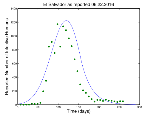
(b) El Salvador - Model (1) is able to capture the overall pattern of the epidemic but with a slightly later peak week.
