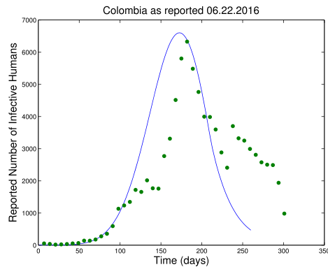
(a) Colombia - Model (1) initially fits the data well but was unable to capture the dynamics observed towards the end of the epidemic.
