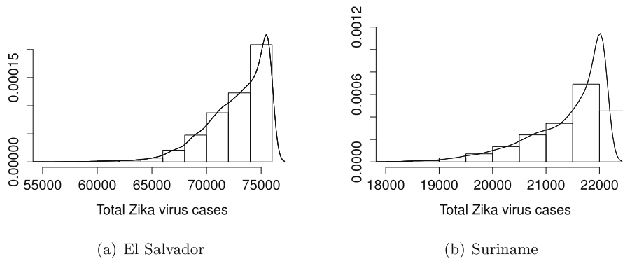
Fig. 11. Histogram and kernel density plot of generated total number of Zika virus cases, both reported and unreported, from the ABC accepted parameter values for El Salvador (a) and Suriname (b).
