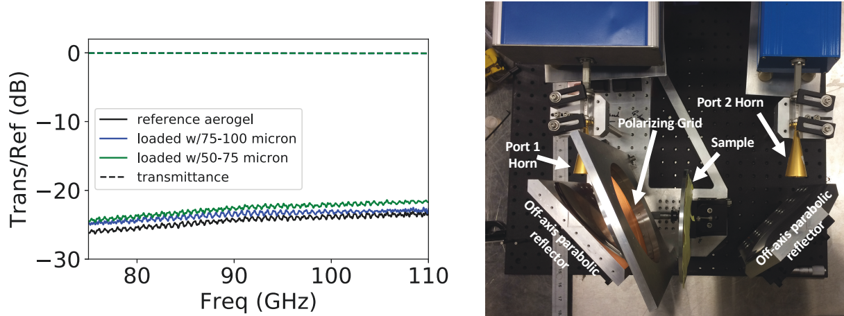
Figure 3. Left : Vector network analyzer measurements of the reflectance (solid lines) and transmittance (dashed lines) of polyimide aerogel samples with no silicon powder (black), 3 \text{ mg/cm}^3 of 50\text{-}75 \mu\text{m} silicon powder (green), and 5 \text{ mg/cm}^3 of 75\text{-}100 \mu\text{m} silicon powder (blue). Right : Photograph of the setup used to make the measurements. Scalar feedhorns both transmit and receive power through the system. Off-axis parabolic reflectors provide a beam waist at approximately the location of the sample and a polarizing wiregrid reduces mode coupling in the setup. The sample is mounted on a linear translation stage.
