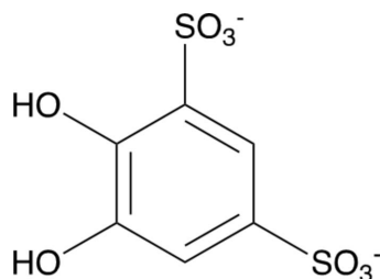
Figure 1 Tiron dianion (4,5-dihydroxy-1,3-benzenedisulfonate).
