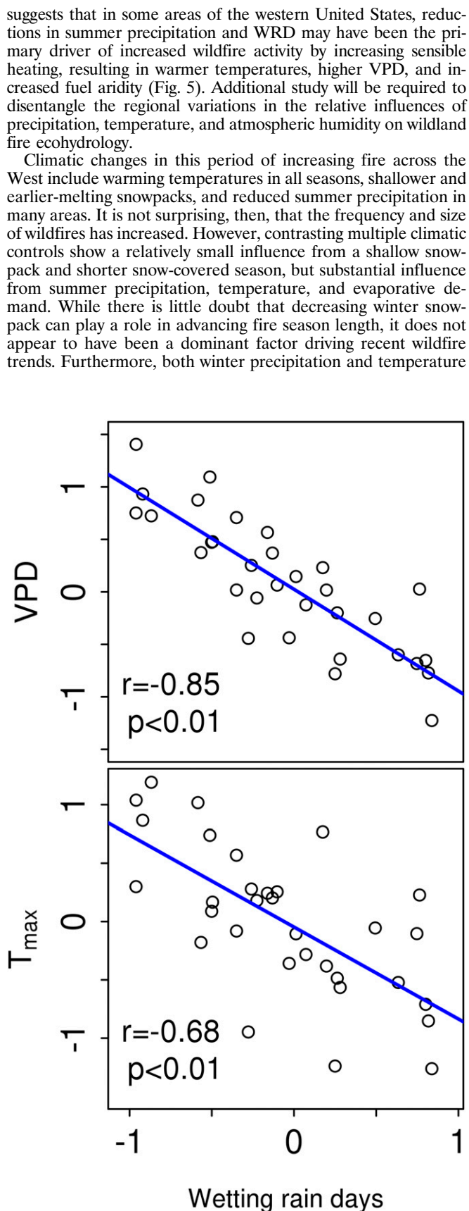
Fig. 5. May–September WRD anomalies correlated with maximum VPD and maximum temperature anomalies for western US forested areas from 1984–2015.
