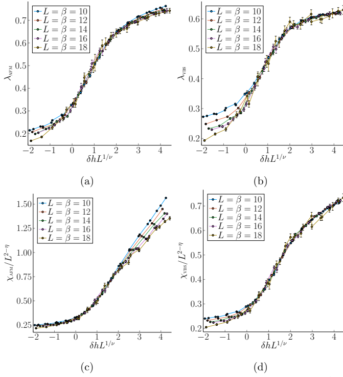
Fig. 4. Finite size scaling analysis of (a) \lambda_{\text{AFM}} (b) \lambda_{\text{VBS}} (c) \chi_{\text{AFM}} and (d) \chi_{\text{VBS}} . In all cases, curve collapse is obtained using the critical coupling h_c = 0.69 , the correlation length exponent \nu = 0.58 . The same anomalous exponent \eta = 1.4 is used to scale both the AFM and VBS fluctuations.
