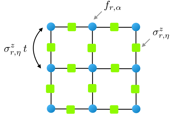
Fig. 1. Lattice model – the fermions f_{r,\alpha} reside on the square lattice sites (blue circles) and the Ising gauge fields, \sigma_{r,\eta}^z , reside on the bonds (green squares). The Ising gauge field determines the sign of the hopping amplitude along the corresponding bond.
