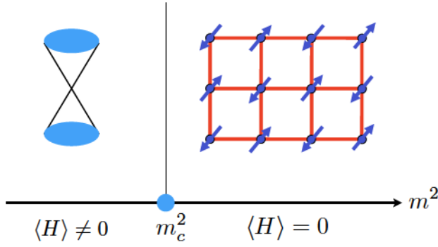
Fig. 5. Higgs mediated confinement transition. For positive Higgs mass, m^2 > 0 , the Higgs field is gapped. The effective field theory is then \text{QCD}_3(N_f = 2) , which confines and spontaneously breaks chiral symmetry, leading to an insulator with AFM order. Conversely, for m^2 < 0 , the Higgs field condenses and reduces the SU_g(2) gauge symmetry down to \mathbb{Z}_2 giving rise to the OSM.
