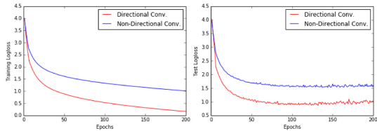
Figure 4: Training logloss (left) and test logloss (right) on 3D Human shapes with directional convolution (red curves) and non-directional convolution (blue curves).
