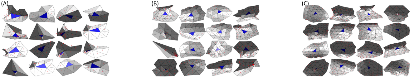
Figure 5: Strongest responses of convolution filters in Conv1 of DCN. The center face of each patch is marked blue and normal of each face is drawn in red. A: Best matches of 1-r \times 1-r filters. B: Best matches of 2-r \times 2-r filters. C: Best matches of 3-r \times 3-r filters.
