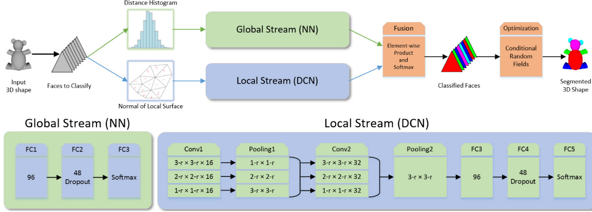
Figure 1: Workflow of our two-stream framework for 3D shape segmentation. Given a 3D shape, we learn representation for each face in the mesh and classify it into the predefined semantic parts. Shape representations are learned with the proposed two-stream framework (DCN and NN) from raw geometric descriptors: face normals and distance histogram. The learned features are fused with an element-wise product and optimized by CRF for segmentation.
