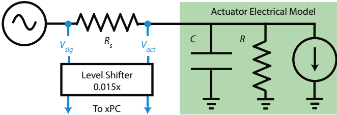
Figure 6. Schematic of lumped parameter electrical model of a single actuator (green) and associated piezoelectric encoder measurement circuit [18].
