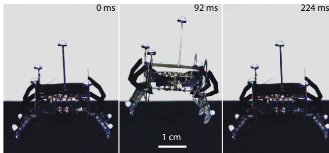
Figure 1. Still frames from the supplementary video ( https://youtu.be/x_wbRQpKukg ) of HAMR-VI executing a vertical jump.
