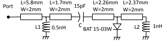
Fig. 3. Device Schematic.
