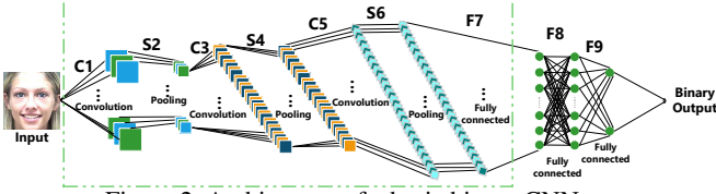
Figure 2. Architecture of a basic binary CNN
