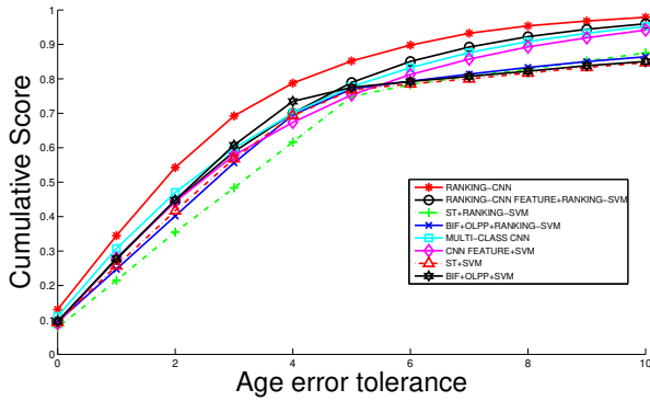
Figure 3. Comparison on Cumulative Score with L in [0, 10] .
