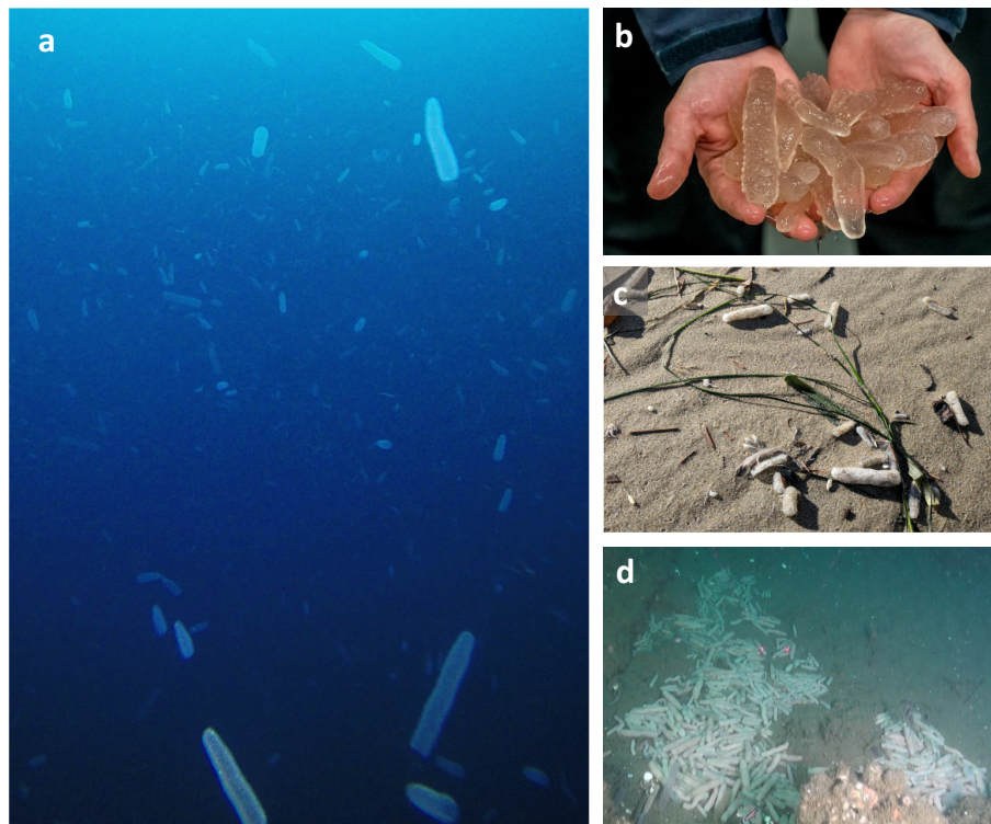
FIG. 1. Pyrosome bloom in the northeast Pacific Ocean. (a) Large densities of Pyrosoma atlanticum observed at ~40 m depth during a February 2018 cruise off of Newport, Oregon, USA (also see Video S1), (b) pyrosome colonies from a net tow on the same cruise (photo by M. Farley), (c) pyrosomes washed up on beach in Newport, November 2017 (photo by A. Rainey) and, (d) dead pyrosomes on the sea floor (~50 m) at Cape Perpetua reef, Oregon, May 2017 (photo by S. Marion).
