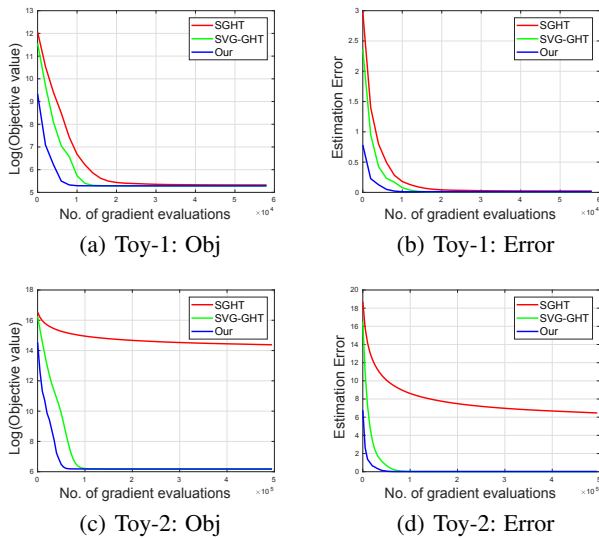
Figure 1: The objective value and estimation error of the model parameter about two synthetic dataset.
