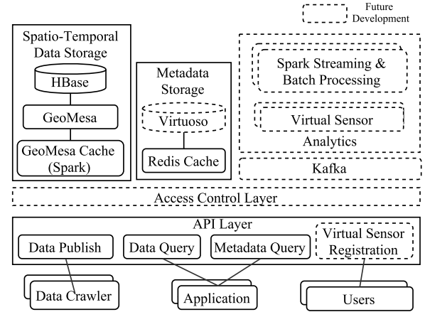
Figure 1: Citadel Architecture.
