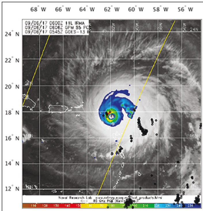
Fig. 7. Hurricane Irma passed over Barbuda on 6 September 2017. Shown here are WWLLN lightning (black circles) and GPM 85-gigahertz PCT brightness temperatures during Irma's maximum intensity as a category 5 storm. Credit: WWLLN-TC
