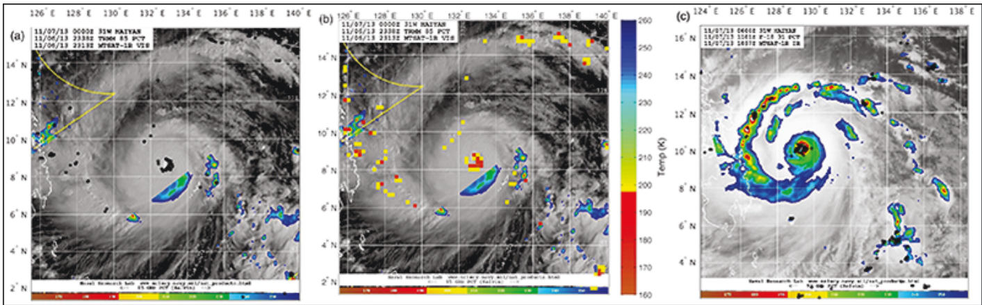
Fig. 5. Reconstruction of satellite data using lightning for Typhoon Haiyan in 2013 at its peak intensity. (a) WWLLN lightning (black circles) and TRMM TMI 85-gigahertz PCT brightness temperatures for a partial pass. (b) WWLLN lightning reconstruction of brightness temperatures for the partial pass. (c) DMSP SSMIS F-18 91-gigahertz PCT brightness temperatures and WWLLN lightning (black circles) 12 hours after the data in Figures 5a and 5b. Images in Figures 5a and 5c are from the WWLLN-TC product.
