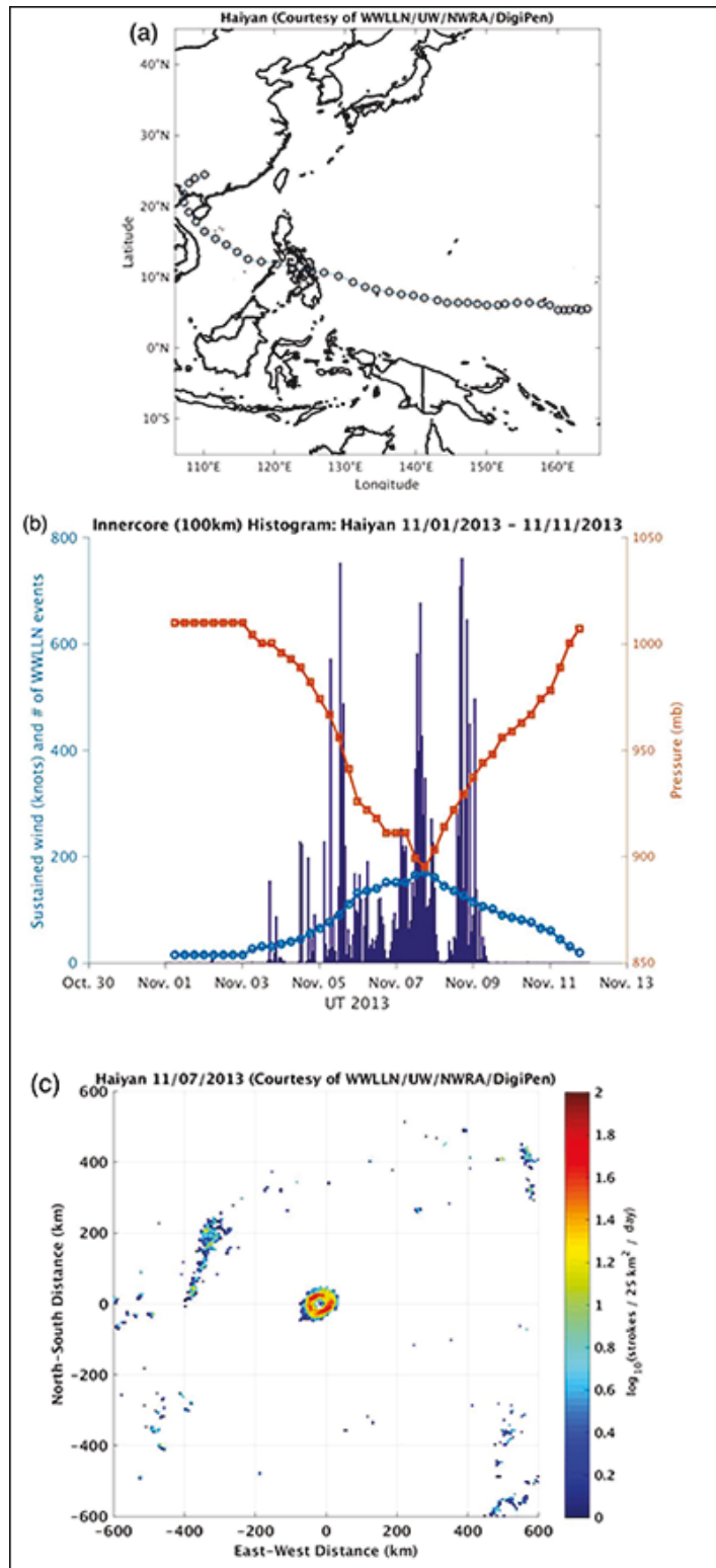
Fig. 2. (a) Storm track for Typhoon Haiyan in 2013. (b) Lightning and intensity histogram, with dark blue bars representing the number of lightning events, wind
