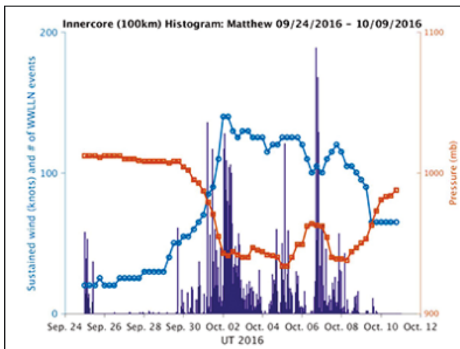
Fig. 3. Histogram of hourly WWLLN lightning, along with wind (blue) and pressure (orange) data, for Hurricane Matthew in 2016. A peak in lightning rate on 6 October precedes rapid weakening of the storm. Credit: WWLLN-TC
