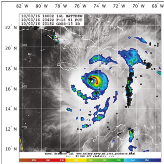
Fig. 4. Results from the WWLLN-TC data product, showing lightning (black circles) and SSMIS 91-gigahertz polarization-corrected temperature (PTC) brightness temperatures (color contours) for Hurricane Matthew in 2016, pinpointing regions of intense convection. Credit: WWLLN-TC
