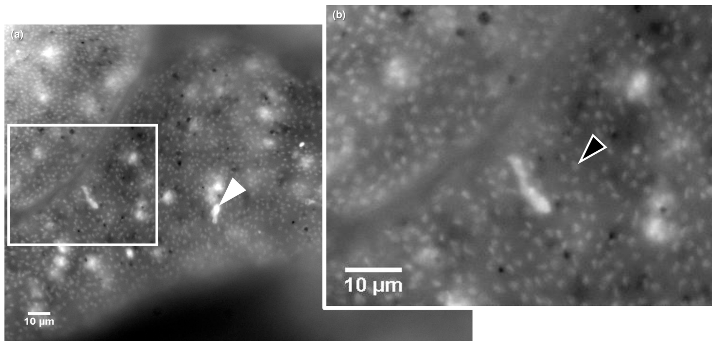
Fig 2. Fluorescence micrograph of a DAPI-stained decalcified N. dutertrei cell. (a) Diffuse autofluorescence can be observed throughout the cytoplasm. The observed ~2 \mu\text{m} diameter structures prevalent throughout the cell are consistent with the presence of picoeukaryotic algae. The white arrowhead denotes an example of the bright spots, 5–10 \mu\text{m} in size that may be food vacuoles containing condensed prey items. The white rectangle denotes the area magnified in (b) where the black arrowhead highlights one of the ~2 \mu\text{m} diameter putative picoeukaryotes.
