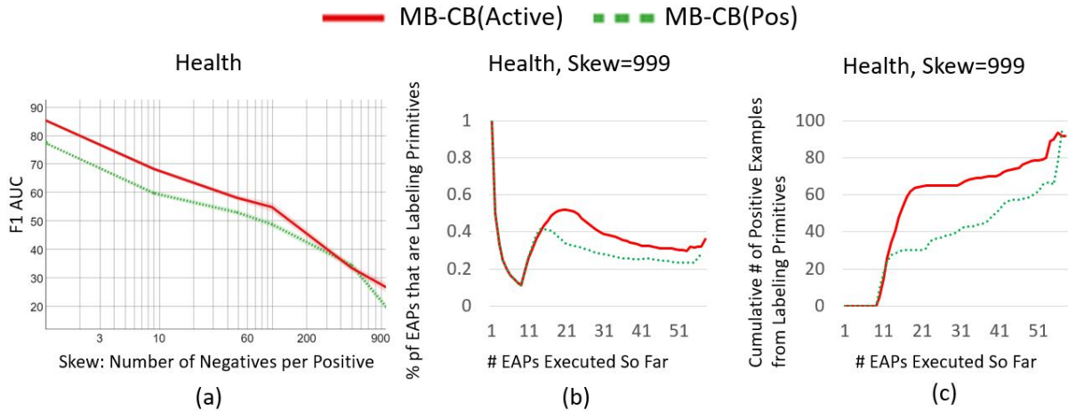
Figure 2: When training classifiers to identify “Health” headlines: (a) MB-CB (Active) outperforms MB-CB (Pos) in all skew settings; (b) when the skew is 999, MB-CB (Active) executes Labeling Primitives more often and Generation Primitives less often than MB-CB (Pos) ; (c) when the skew is 999, MB-CB (Active) surprisingly obtains more positive examples from Labeling Primitives than does MB-CB (Pos) . We find similar results for the other three domains.
