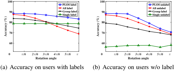
Figure 8. Accuracy comparison on the synthetic dataset w.r.t. the rotation angles
