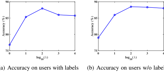
Figure 7. Accuracy comparison on HAR dataset w.r.t. the model parameters
