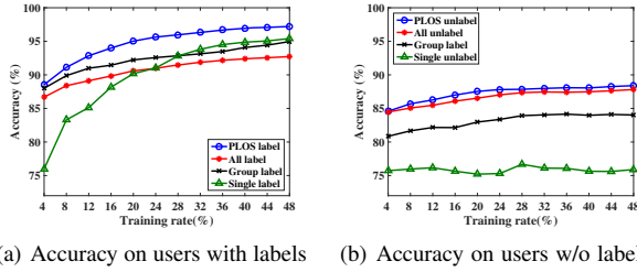
Figure 4. Accuracy comparison on body sensor dataset w.r.t. the percentage of labeled data on the users who provide labels
