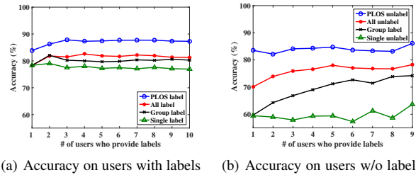
Figure 9. Accuracy comparison on synthetic dataset w.r.t. the number of users who provide labels
