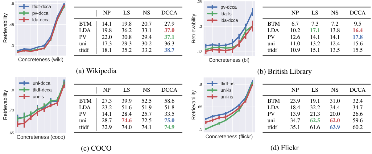
Figure 5: Concreteness scores versus retrievability (plotted) for each dataset, along with Recall at 1% (in tables, higher is better) for each algorithm combination. Tables give average retrieval performance over 10-fold cross-validation for each combination of NLP/alignment algorithm; the best , second best , and third best performing combinations are bolded and colored. The concreteness versus retrievability curves are plotted for the top-3 performing algorithms, though similar results hold for all algorithms. Our concreteness scores and performance are positively correlated, though the shape of the relationship between the two differs from dataset to dataset (note the differing scales of the y-axes). All results are for RN-ImageNet; the similar I3-OpenImages results are omitted for space reasons.
