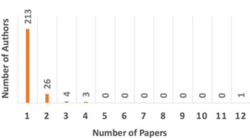
Figure 2. Distribution of the number of papers published per HCD+D author (average = 1.22).
