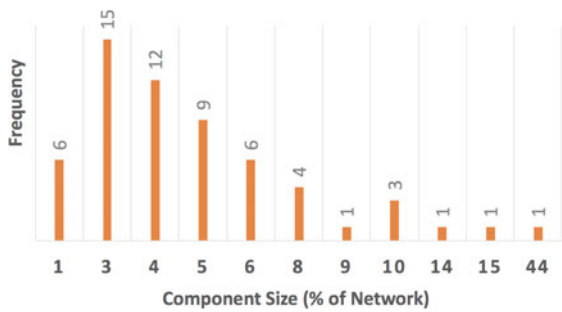
Figure 6. Distribution of connected component (sub-community) sizes (average = 4.26).
