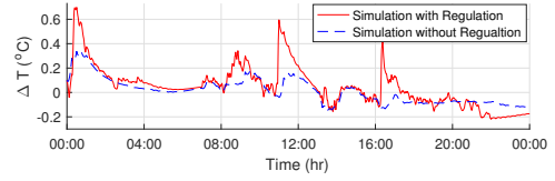
Fig. 6. Temperature deviation trajectory with symmetric regulation
