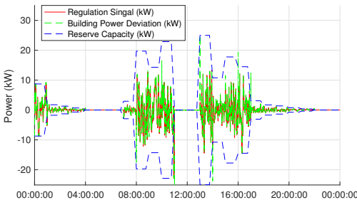
Fig. 5. Frequency regulation performance for a whole day
