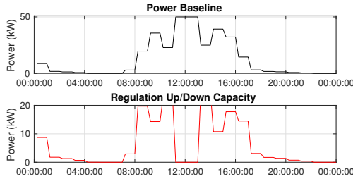
Fig. 3. Frequency Regulation up/down capacity and power baseline
