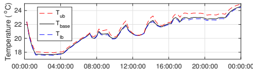
Fig. 4. Expected temperature curves
