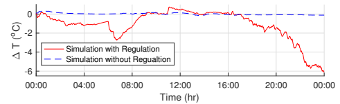
Fig. 7. Temperature deviation trajectory with asymmetric regulation
