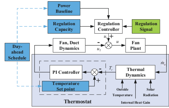
Fig. 2. Schematics of the regulation signal tracking control
